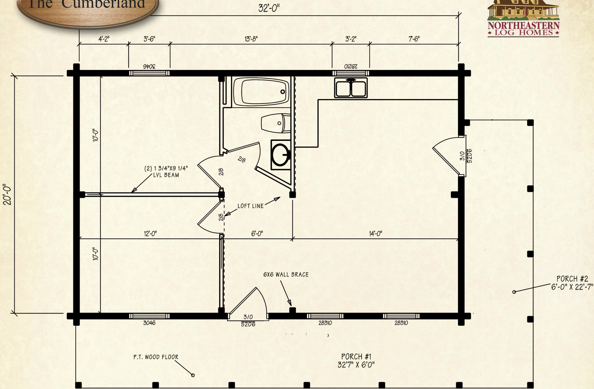
Cumberland plan above shown with optional interior partitions
