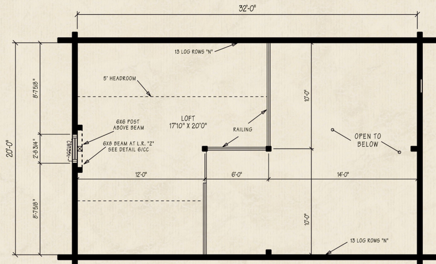
Cumberland plan above shown with optional interior partitions
